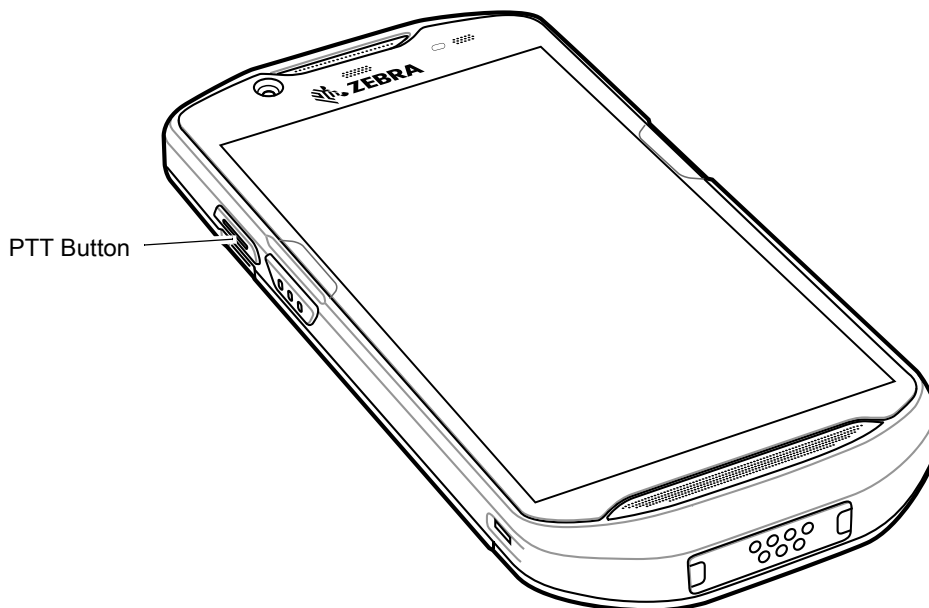
Figure 70 PTT Button
